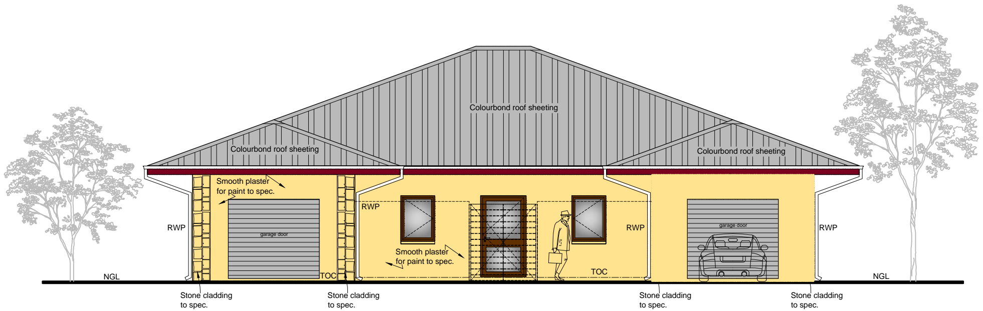
ELEVATION 1-1
